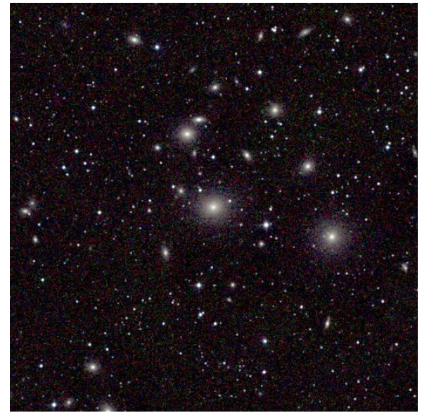
NGC 1275
